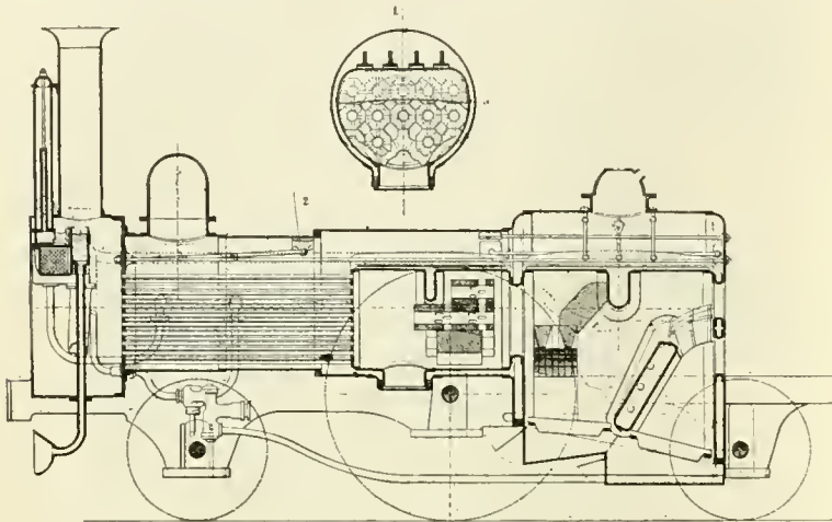
BEATTIE'S SMOKE PREVENTING BOILER. FIG. 53.
